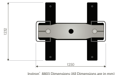
Instron® 8803 Dimensions (All Dimensions are in mm)
